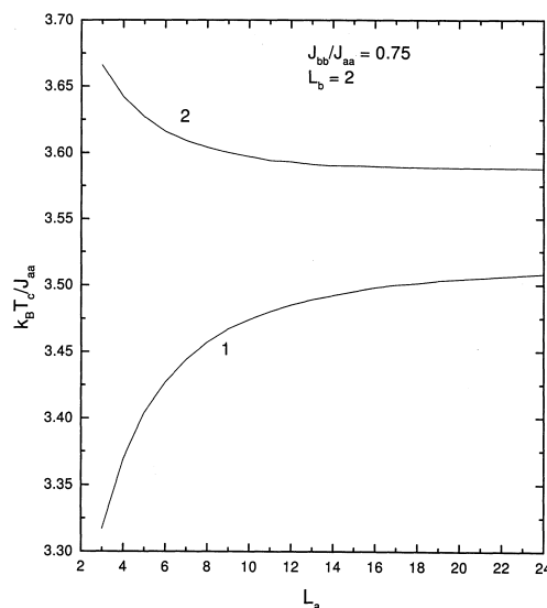
FIG. 5. The dependence of the Curie temperature k_B T_c(L_a) / J_{aa} on the layer-number L_a of the slab A for fixed values of L_b = 2 and J_{bb} / J_{aa} = 0.75 . The number accompanying each curve denotes the value of J_{ab} / J_{aa} .
