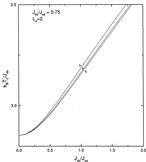
FIG. 2. The Curie temperature k_B T_c / J_{aa} versus J_{ab} / J_{aa} for fixed values of L_a = 2 and J_{bb} / J_{aa} = 0.75 . The number accompanying each curve denotes the value of L_b .
