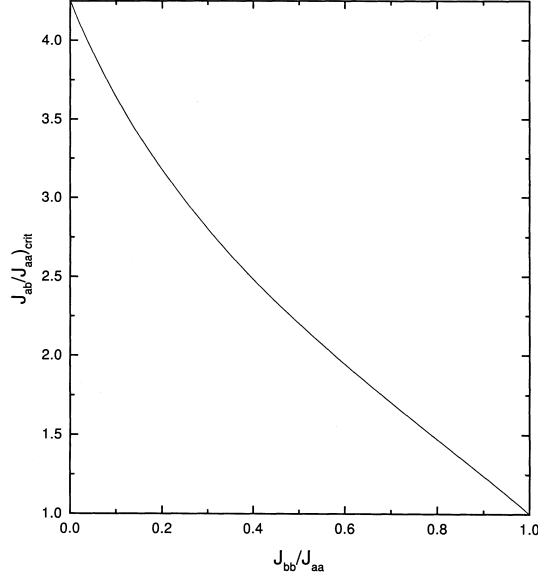
FIG. 6. The reduced critical interface exchange interaction (J_{ab}/J_{aa})_{crit} on the reduced exchange interaction J_{bb}/J_{aa} .
