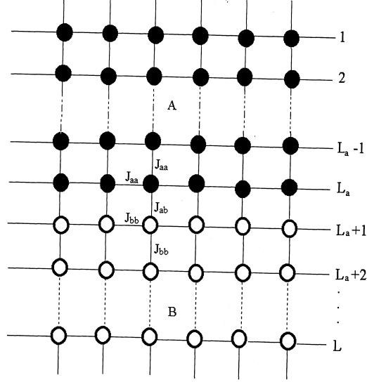
FIG. 1. Sketch of a unit cell of the superlattice.
