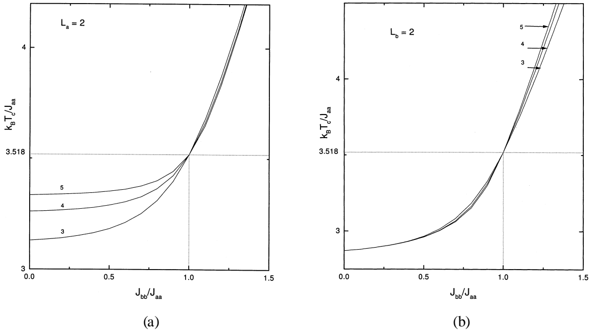
FIG. 7. a(b). The dependence of the Curie temperature on J_{bb}/J_{aa} for L_a(L_b) = 2 , J_{ab} = (J_{aa} + J_{bb})/2 with different values of L_b(L_a) = 3, 4 and 5 denoted by the numbers.
