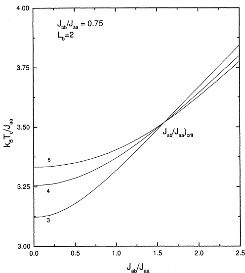
FIG. 4. The Curie temperature k_B T_c / J_{aa} versus J_{ab} / J_{aa} for fixed values of L_b = 2 and J_{bb} / J_{aa} = 0.75 . The number accompanying each curve denotes the value of L_a .
