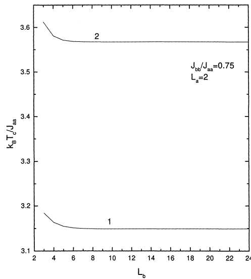
FIG. 3. The dependence of the Curie temperature k_B T_c(L_b) / J_{aa} on the layer-number L_b of the slab B for fixed values of L_a = 2 and J_{bb} / J_{aa} = 0.75 . The number accompanying each curve denotes the value of J_{ab} / J_{aa} .
